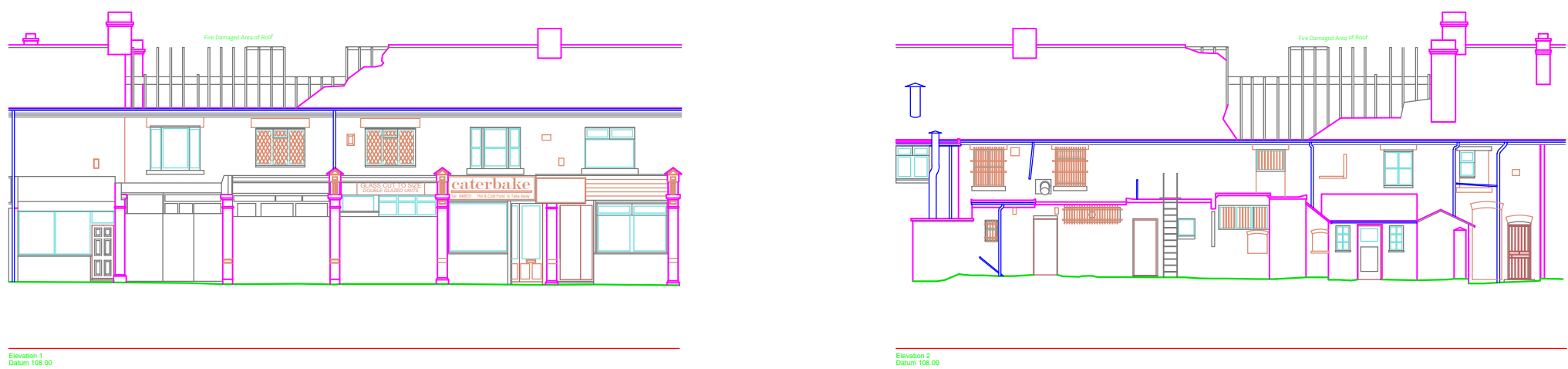
Figure 3: Front and rear elevations of retail units, showing extent of damage to roof and roof structure.
